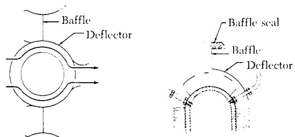
FIGURE 6-34. Heat dissipation.
