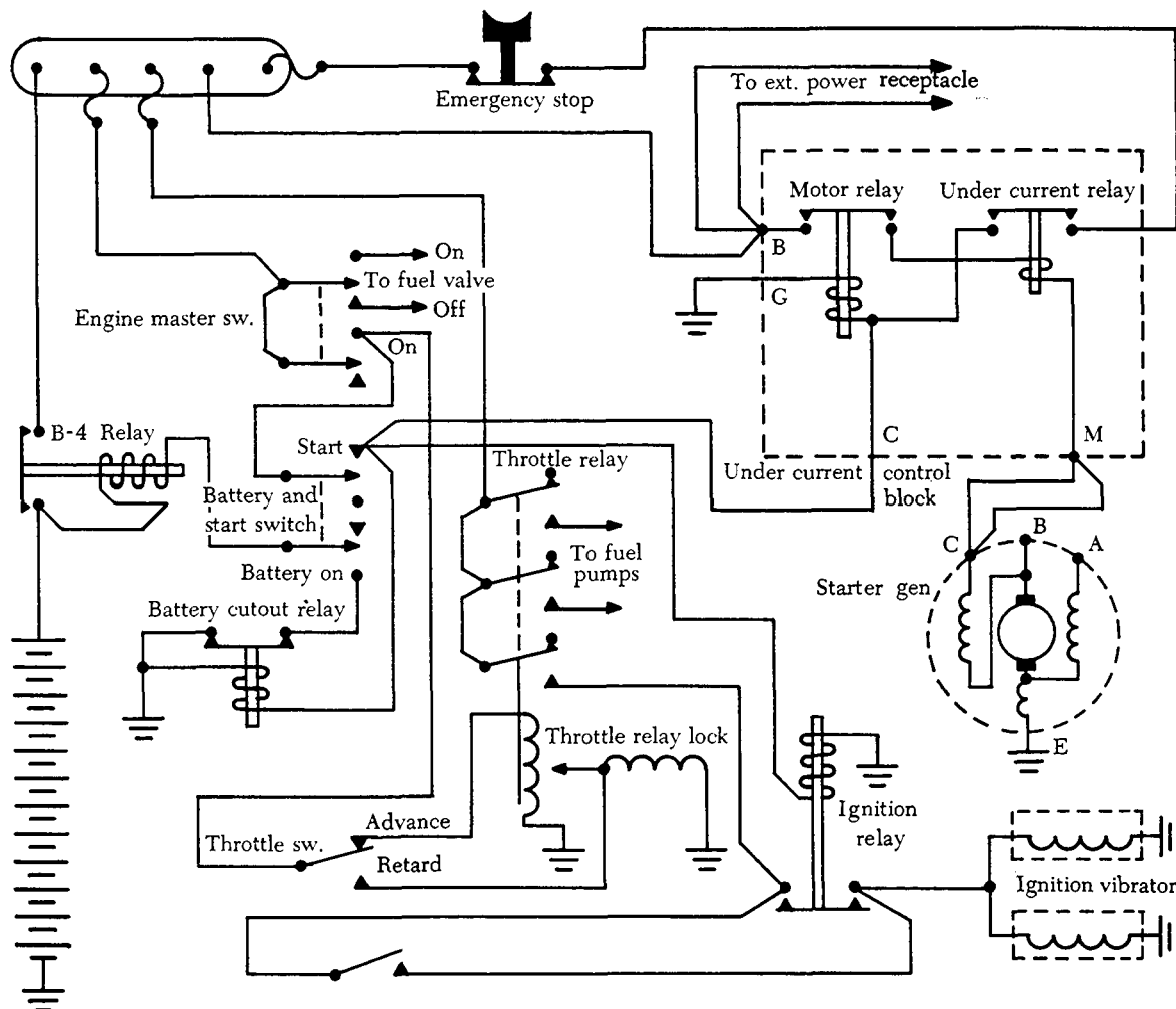
FIGURE 5-15. Starter-generator circuit.
