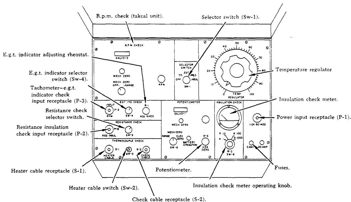
FIGURE 10-71. Jetcam analyzer instrument compartment.
