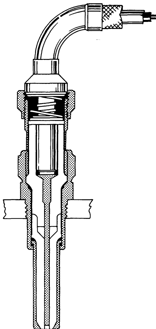
FIGURE 4-79. Constrained-gap igniter plug.
