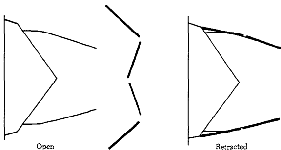
FIGURE 2-38. Mechanical blockage thrust reverser.
