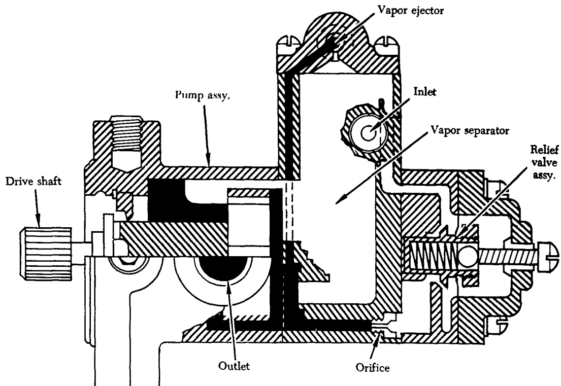
FIGURE 3-35. Fuel-injection pump.
