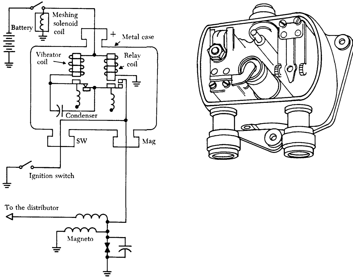
FIGURE 4-22. Induction vibrator.
