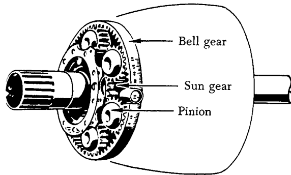
Spur-planetary
