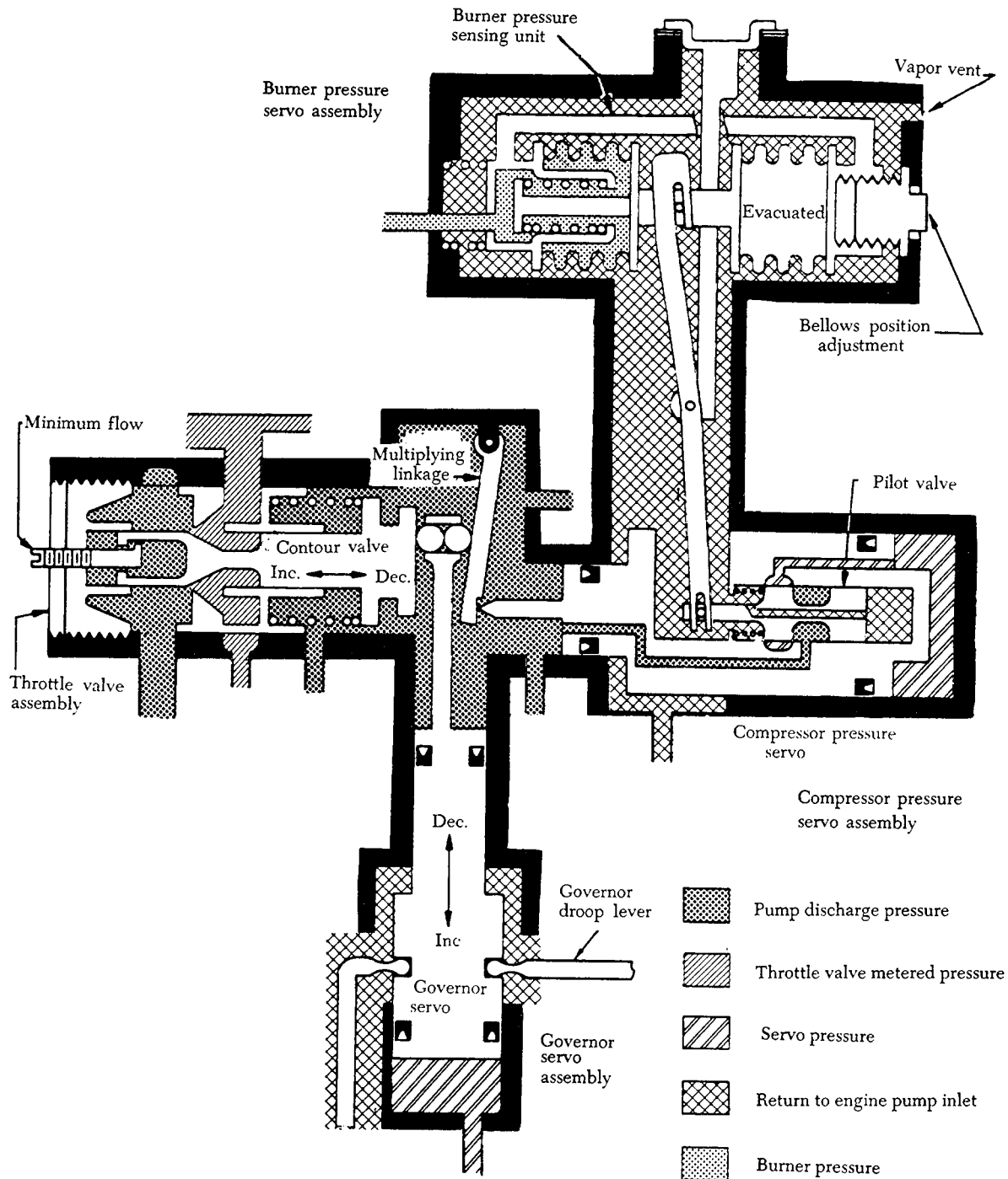
FIGURE 3-50. Computing system.
