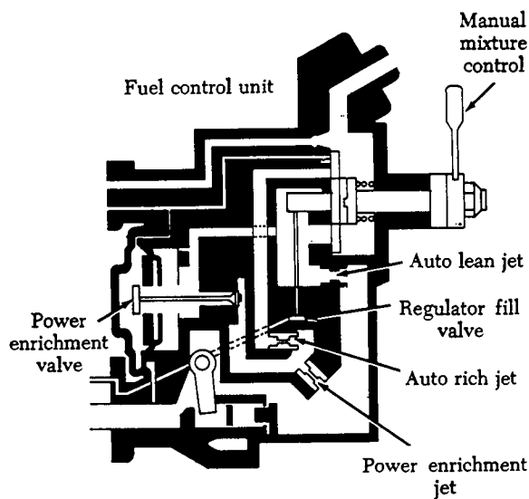
FIGURE 3-19. Fuel control unit.
