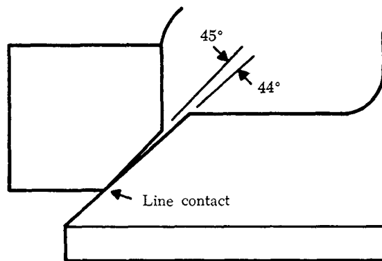
FIGURE 10-14. Interference fit of valve and valve seat.
