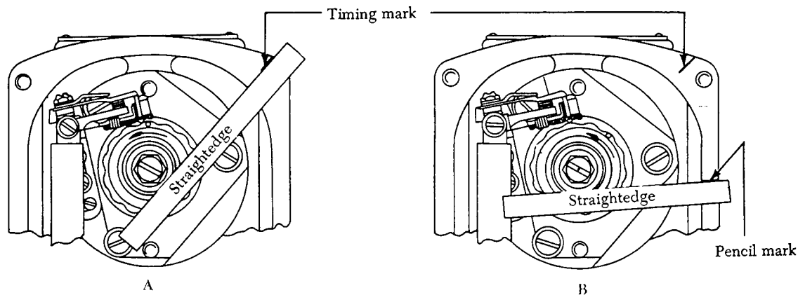
FIGURE 4-44. Aligning straightedge.
