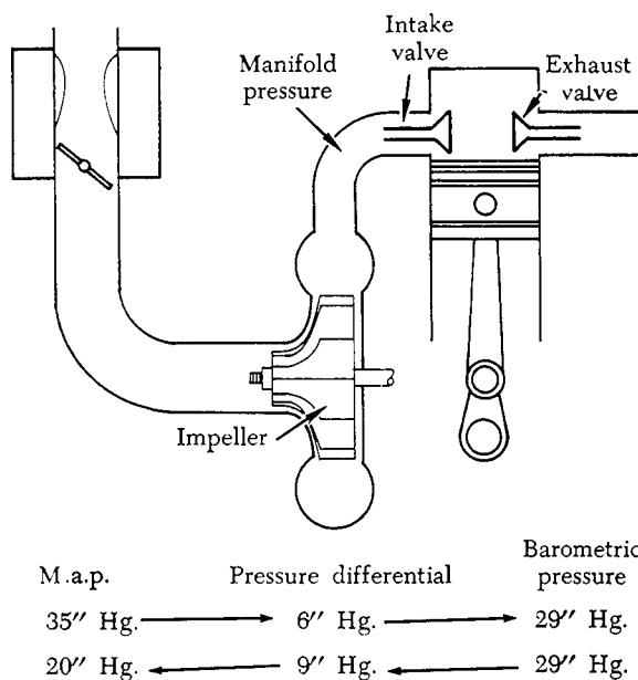
FIGURE 10-40. Effect of valve overlap.
