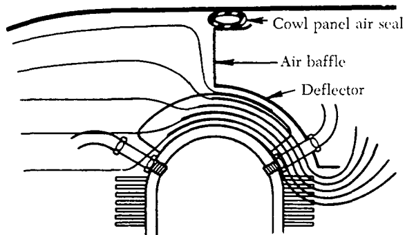
FIGURE 6-44. Cylinder head baffle and deflector system.
