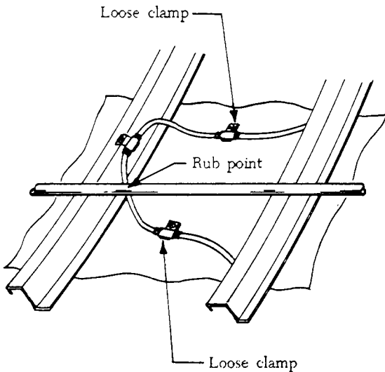
FIGURE 9-19. Rubbing interference.
