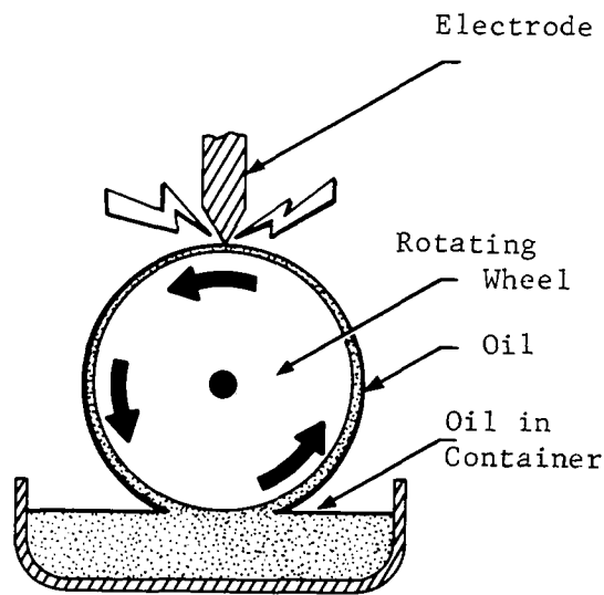
FIGURE 10-74. Oil Sample
