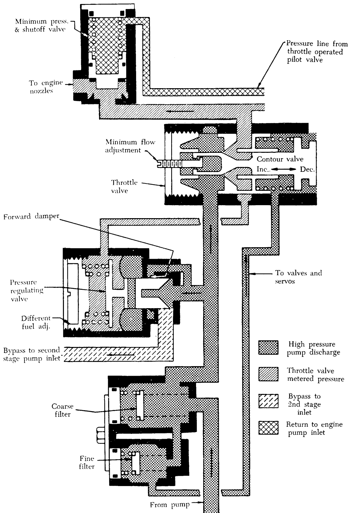
FIGURE 3-48. Metering system.
