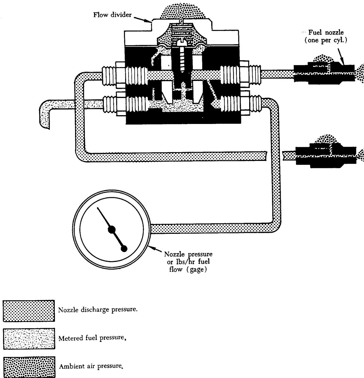
FIGURE 3-34. Flow divider.
