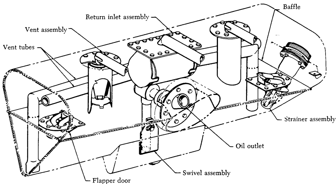
FIGURE 6-23. Oil tank.
