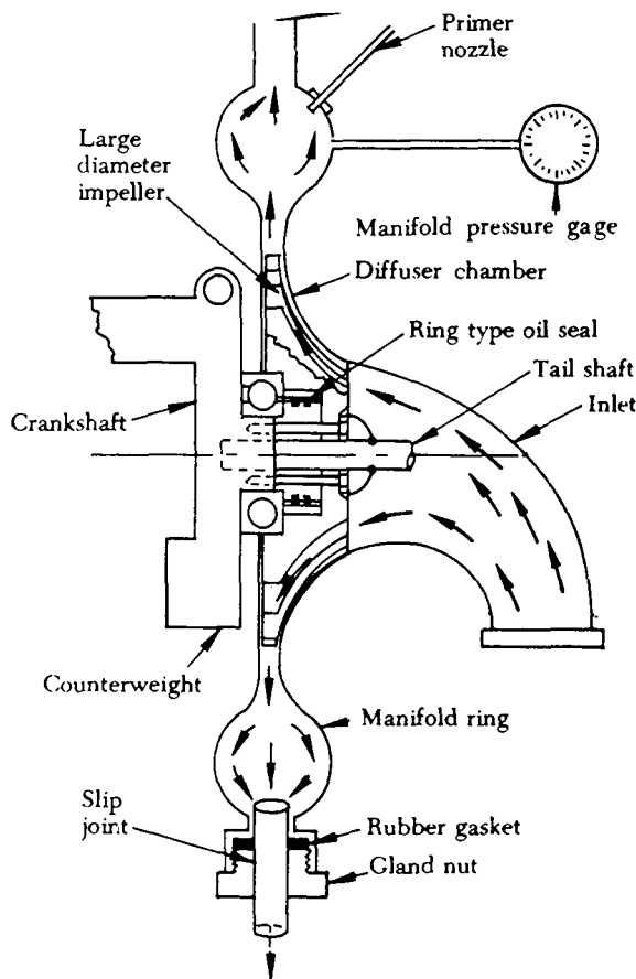
FIGURE 2-4. Distribution impeller arrangement used on a radial engine.
