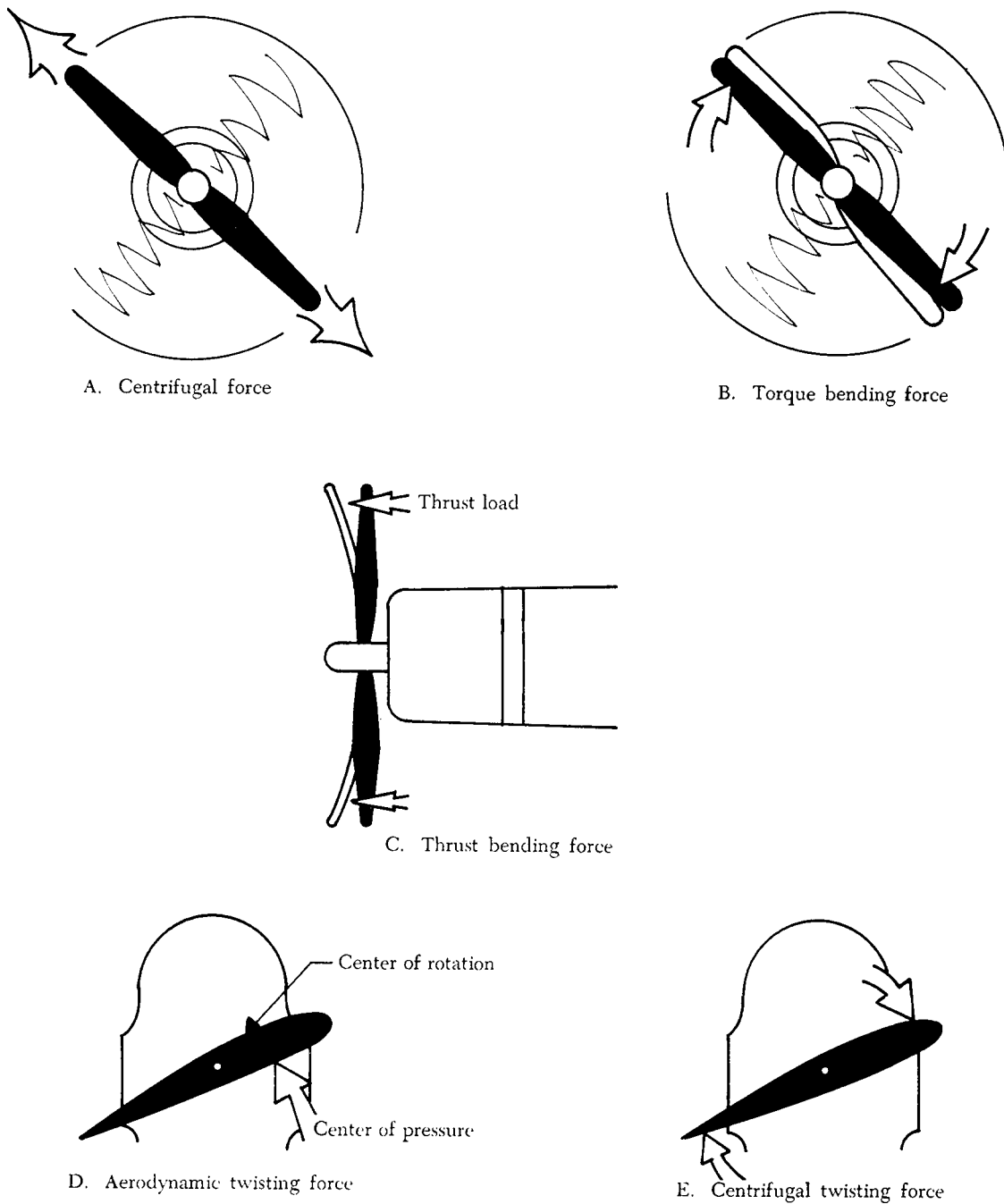
FIGURE 7-5. Forces acting on a rotating propeller.
