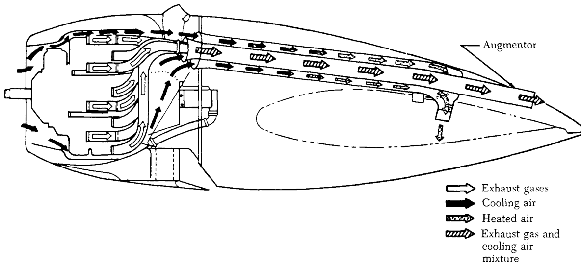
FIGURE 6-36. Augmentor.
