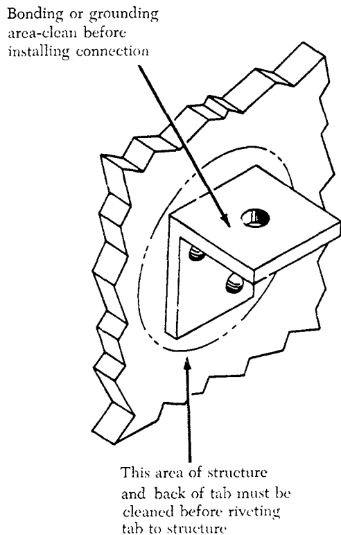
FIGURE 4-116. Bonding or grounding tab riveted to structure.
