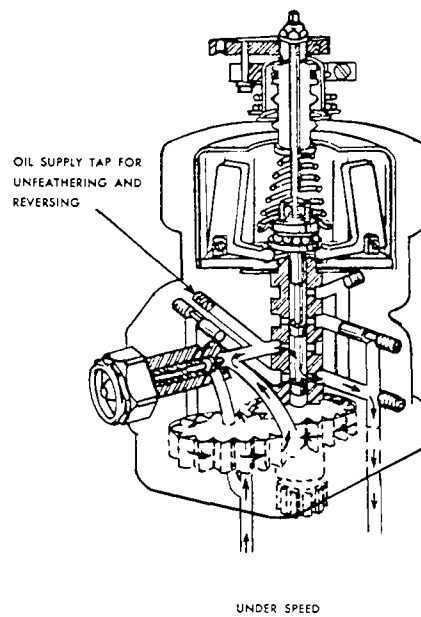
FIGURE 7-16. Woodward Governor X210,000 Series
