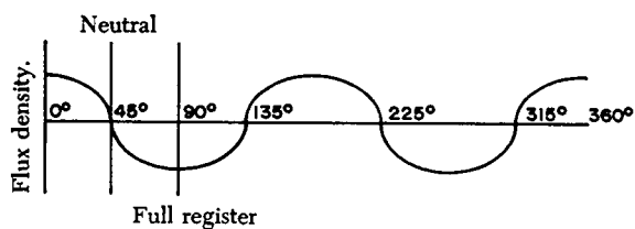
FIGURE 4-3. Change in flux density as magnet rotates.
