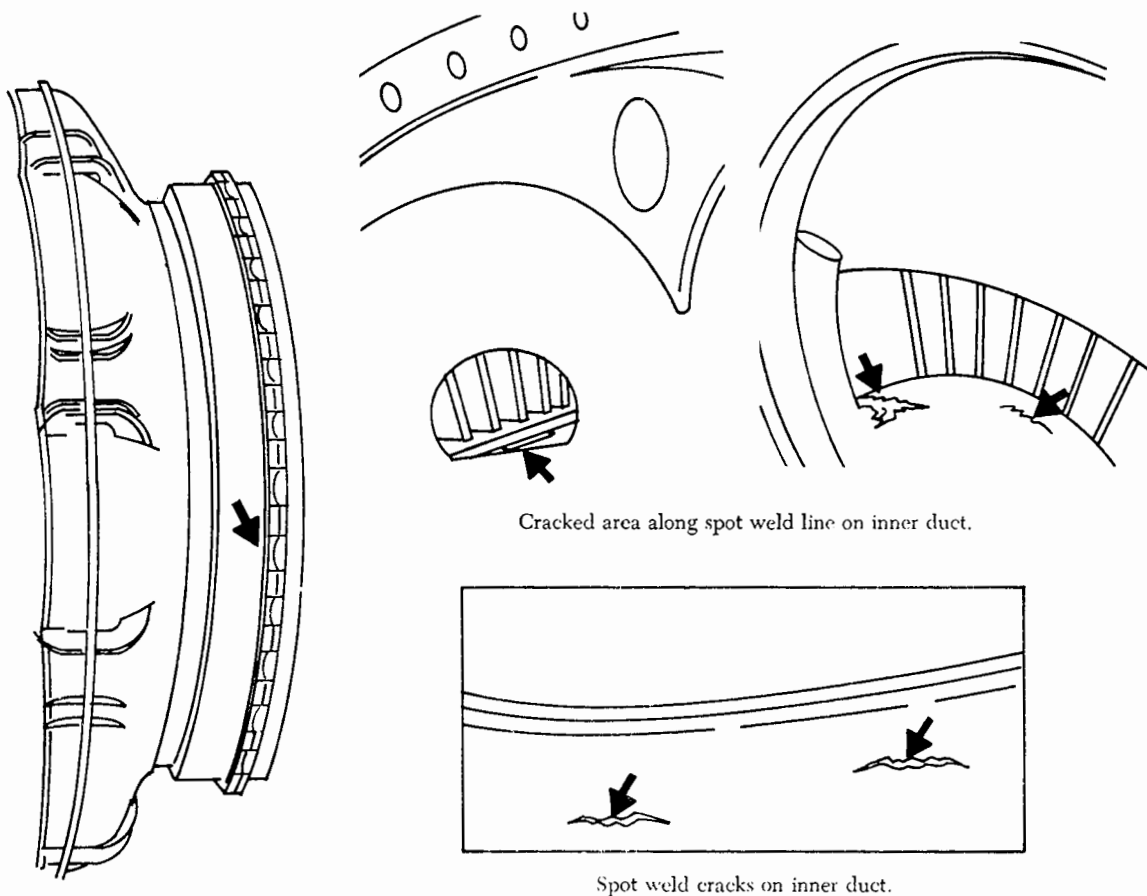
FIGURE 10-65. Typical turbine nozzle assembly defects.
